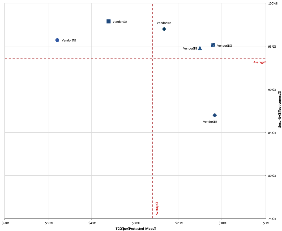
Figure 3 – Example SVM
